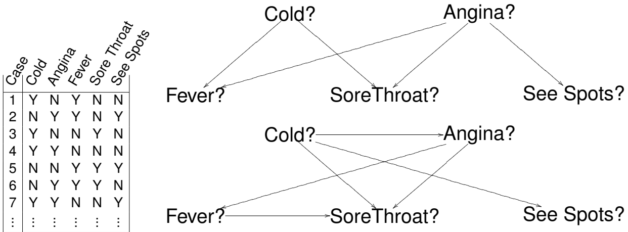
Figure 12: Different bayesian network structures.
