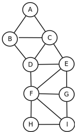
(a) Markov Network
