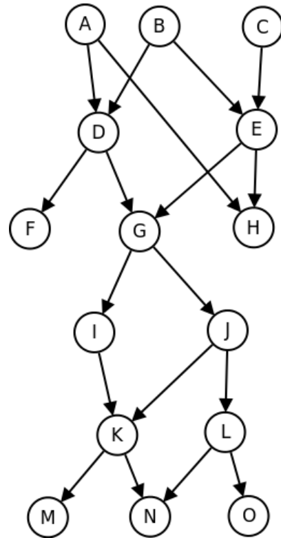
(b) Bayesian Network
