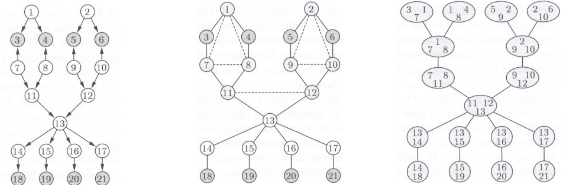
Figure 5: a) Example Bayesian network, b) triangulated moral graph, c) join tree [BK02, p. 127, 129].
