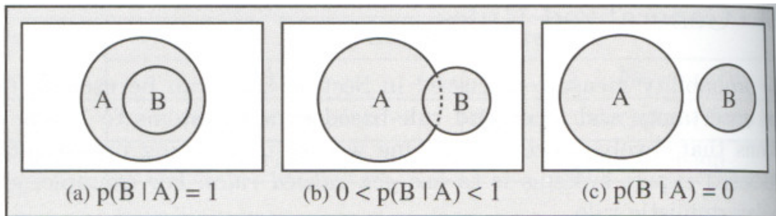
Figure 1: Types of uncertain implications [CGH97, p. 86].
