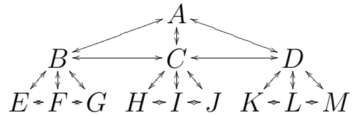
Figure 12: Sitegraph.
