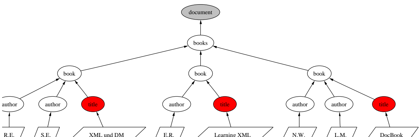
Figure 11: Result of XPath query /descendant-or-self::title .
