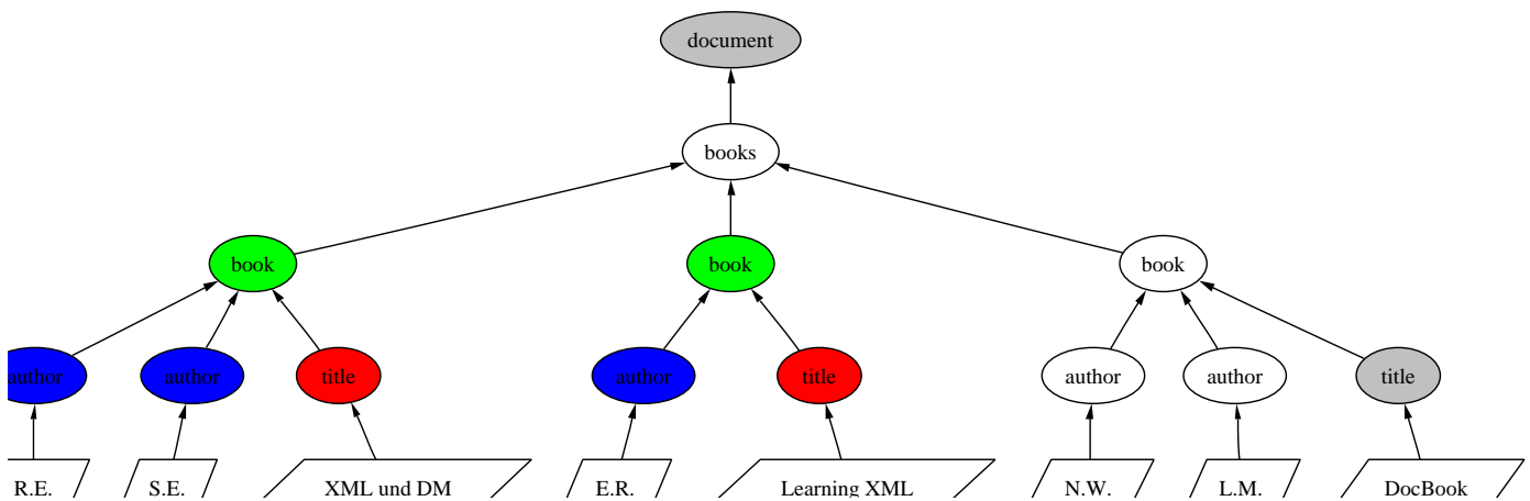
Figure 14: Result of XPath query /descendant-or-self::title[contains(string(),"XML")]/parent::node()/child::auth
