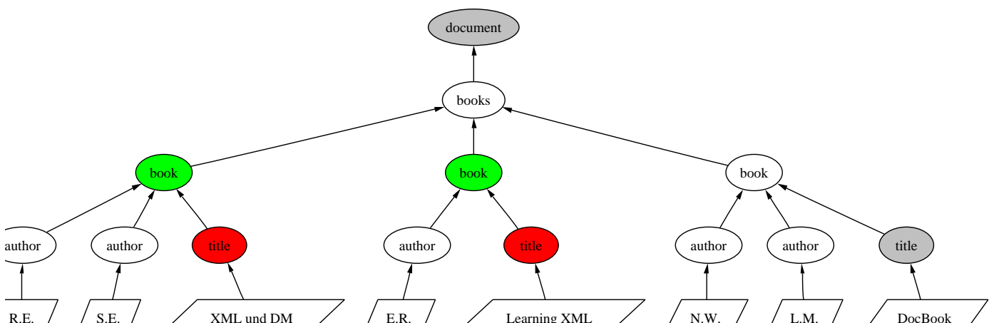
Figure 13: Result of XPath query /descendant-or-self::title[contains(string(.),"XML")]/parent::node() .
