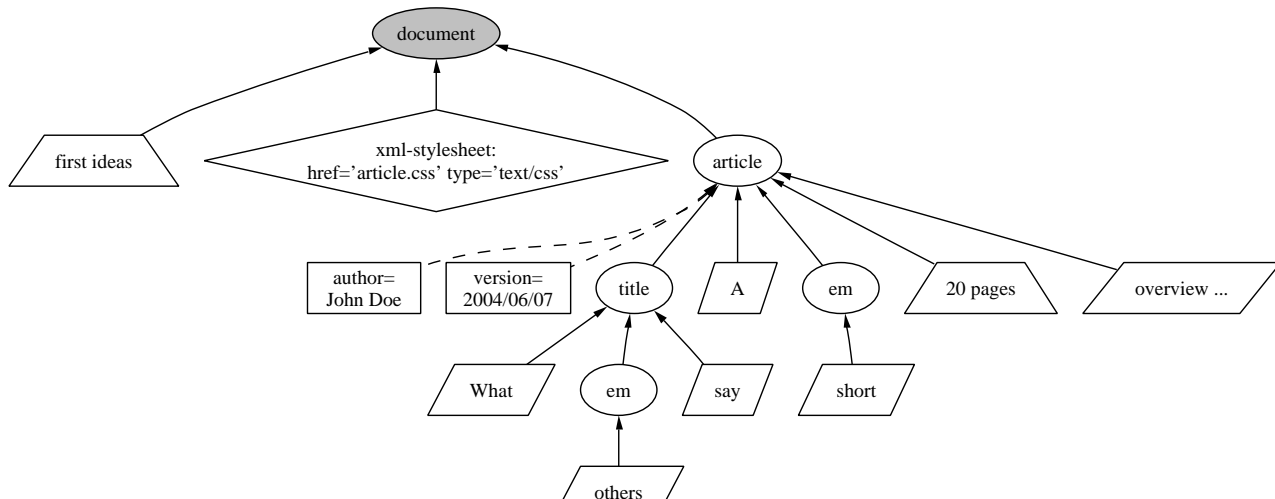
Figure 4: Document tree of the sample document.
