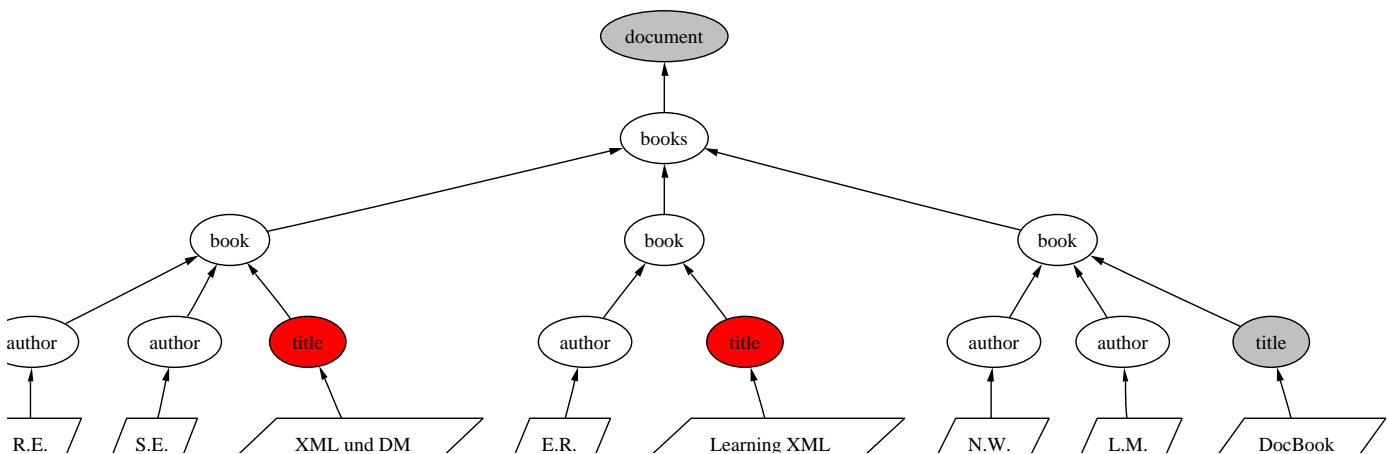
Figure 12: Result of XPath query /descendant-or-self::title[contains(string(.),"XML")] .
