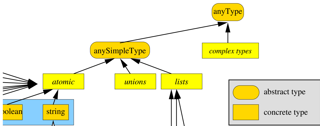
Figure 1: Abstract basetypes in XML Schema type hierarchy.
