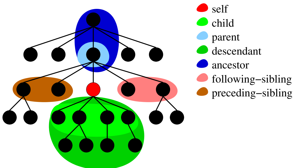
Figure 8: Following-sibling and preceding-sibling axis.
