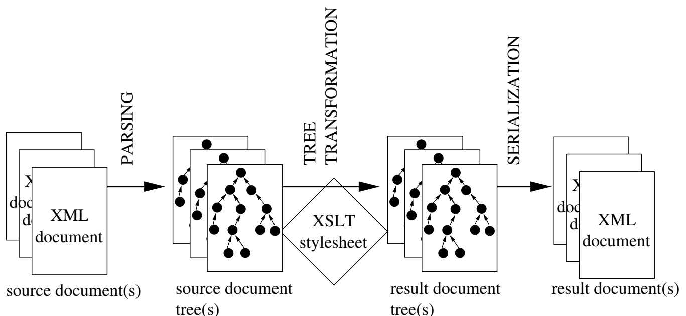
Figure 1: XSLT Processing Model.
