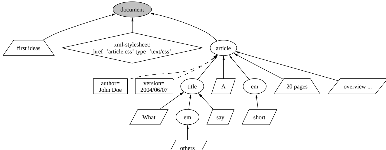
Figure 3: Source Tree.
