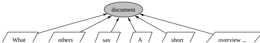
Figure 6: Result Tree.
