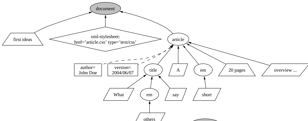
Figure 8: Source Tree.
