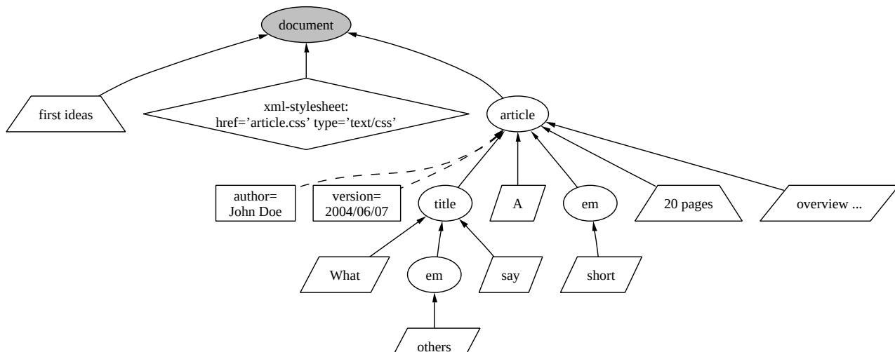
Figure 5: Source Tree.
