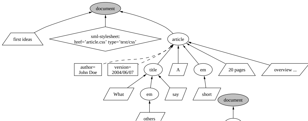
Figure 11: Source Tree.
