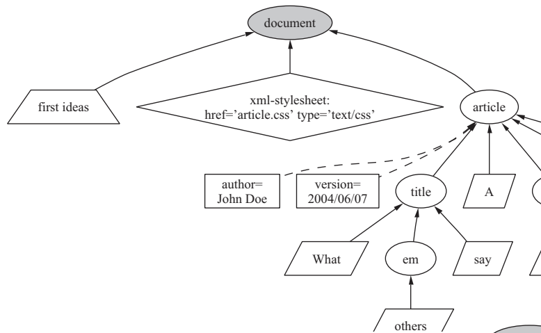
Figure 8: Source Tree.
