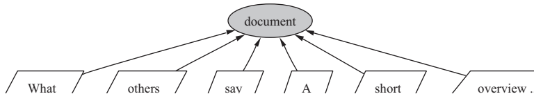
Figure 6: Result Tree.
