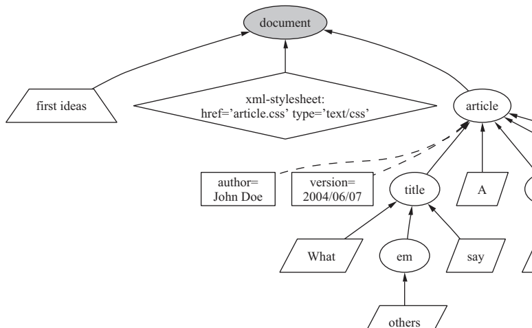
Figure 5: Source Tree.
