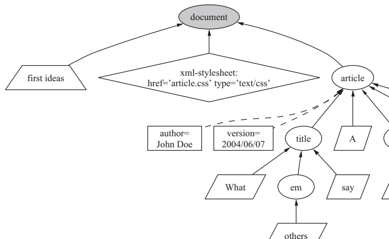
Figure 3: Source Tree.
