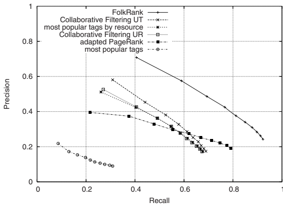
Fig. 2. Recall and Precision for Last.fm p -core at level 10
