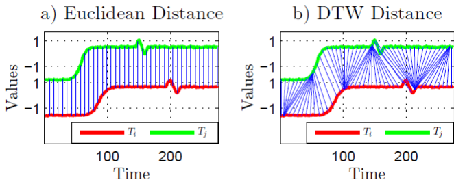
Figure 1: Illustrating DTW
