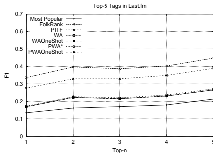
Fig. 4. New user problem Last.fm.
