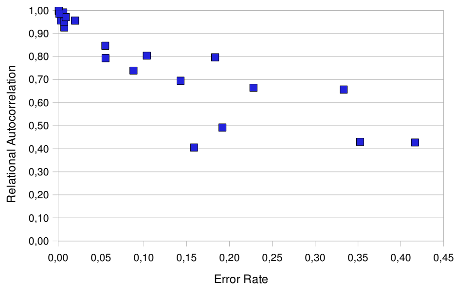
Relational Autocorrelation vs. Error Rate
